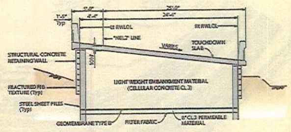
RETAINING WALL SECTION
