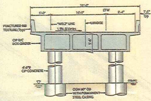
TYPICAL SECTION
