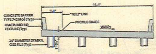
REINFORCED SLAB SECTION
